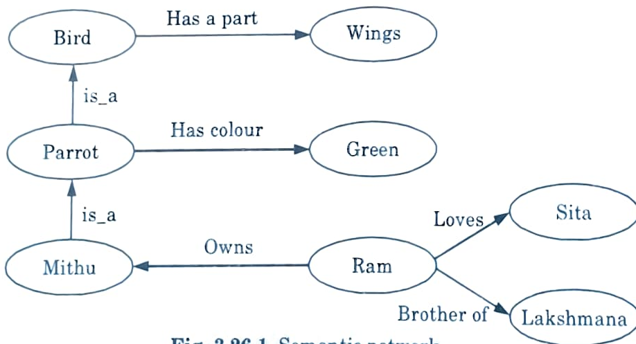
Fig. 3.26.1. Semantic network.
