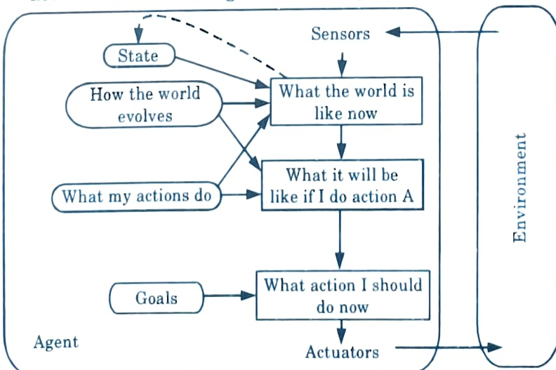
Fig. 1.7.4. Goal-based agent.
