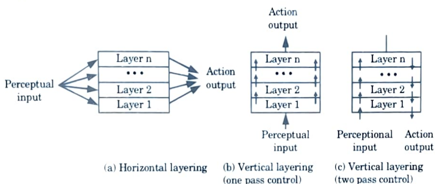
Fig. 4.6.1. Layered agent architecture types.
