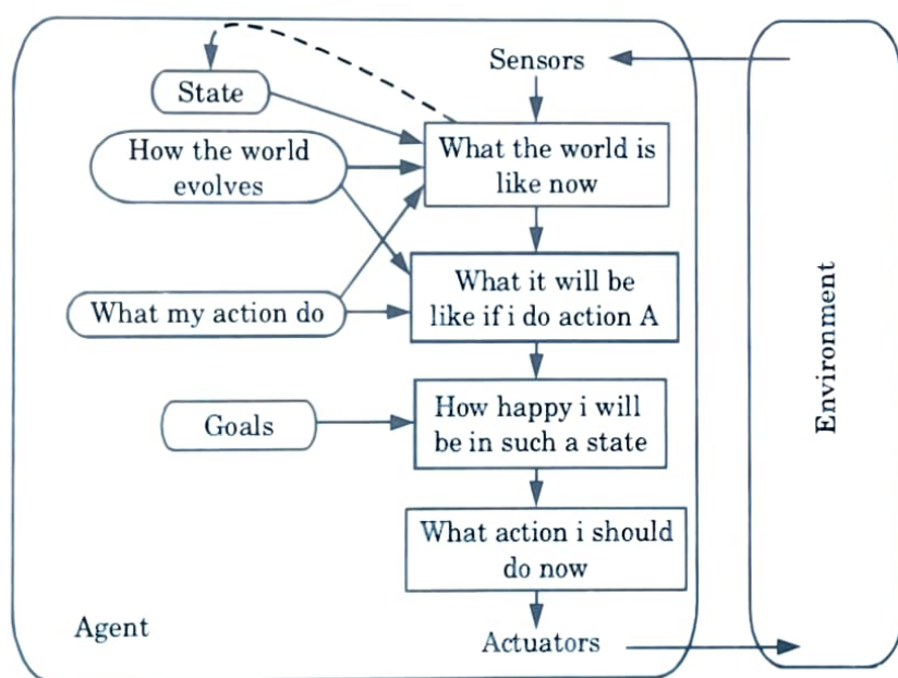
Fig. 1.7.5. Utility-based agent.
